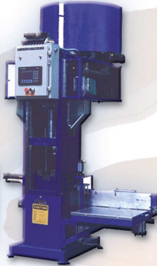
Model P4/P6 70 – 240 Ton Preformer Single or Dual Layer
