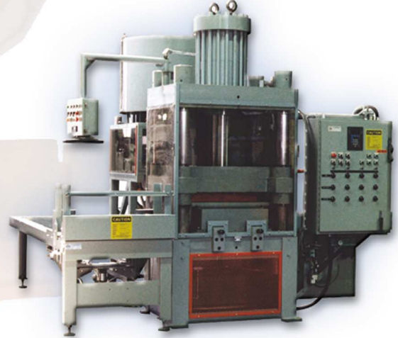
Model BF4 up to 300 Ton Preformer with up to 8 Separate Weighings per Mold
